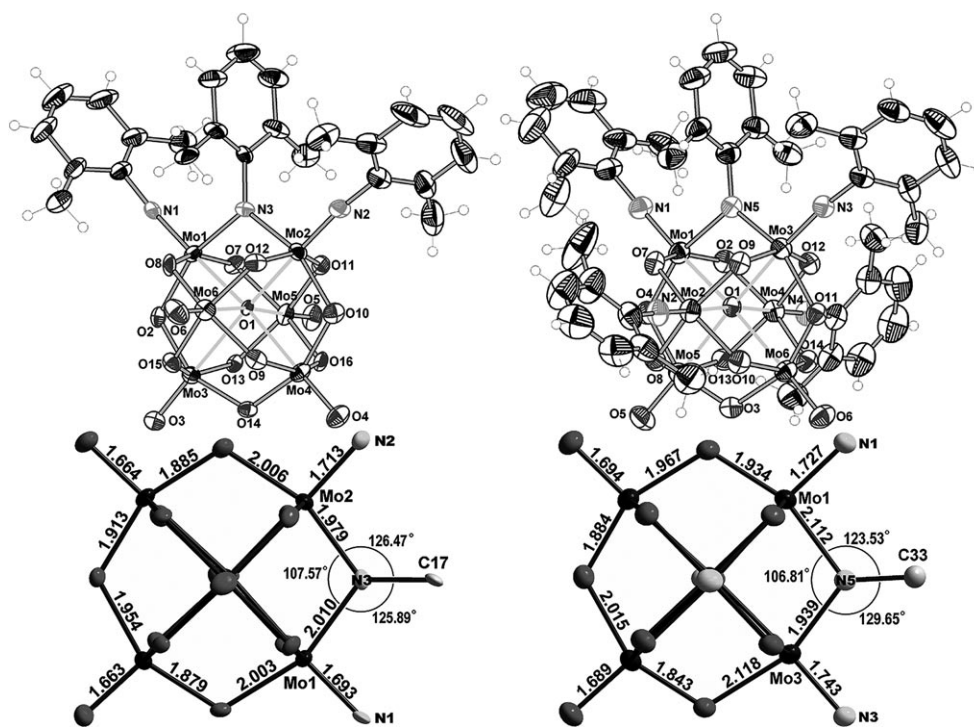
Figure 1. ORTEP showing of the cluster anions 3-Ar-III (left) and 5-Ar-II (right). Thermal ellipsoids are set at 25% probability. Selected bond lengths and angles are given in the depictions of the cores (bottom).
