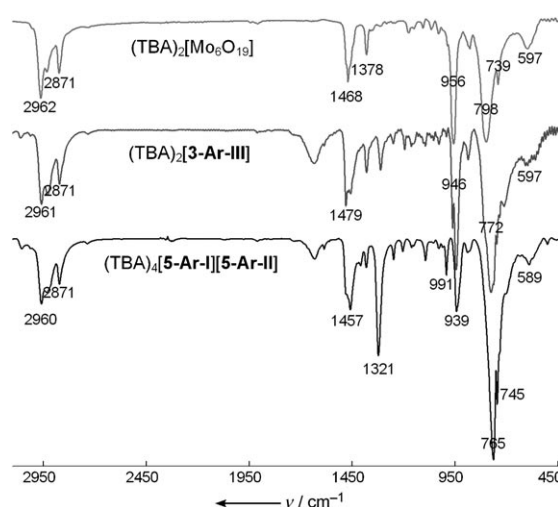
Figure 3. IR spectra of (\text{TBA})_2[\text{Mo}_6\text{O}_{19}] , (\text{TBA})_2[\mathbf{3-Ar-III}] , and (\text{TBA})_4[\mathbf{5-Ar-I}][\mathbf{5-Ar-II}] .
